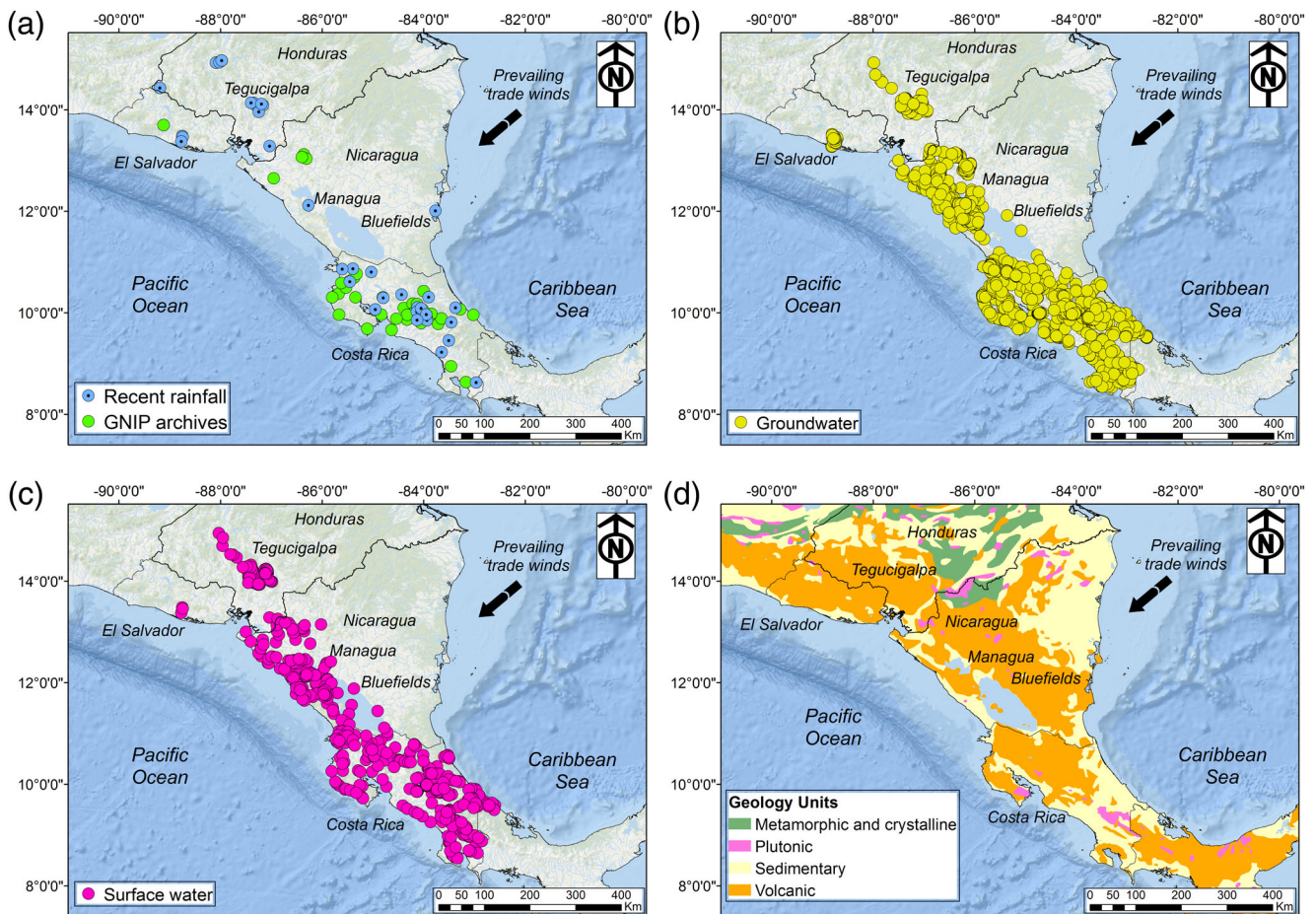
FIGURE 3 Spatial distribution of rainfall, groundwater, and surface water sampling sites across the Central American Isthmus. (a) Recent (2013–2018) rainfall monitoring sites (mostly daily and weekly sampling frequencies; blue circles) and historical GNIP sites [green dots]. (b) Distribution of groundwater sampling sites (light green dots). (c) Distribution of surface water sampling sites (pink dots). (d) Main geological units across Central America. GNIP, Global Network of Isotopes in Precipitation
