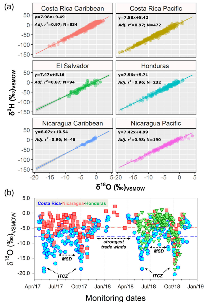
FIGURE 5 Stable isotope variations of rainfall in Central America. (a) Local meteoric water lines (LMWLs) by country and governing rainfall domain (Caribbean vs. Pacific). All regressions are significant with a p -value < .001 . LMWLs include only recent (2013–2018) isotope measurements (mostly daily and weekly sampling frequencies) for comparison purposes. (b) \delta^{18}\text{O} time series (2016–2018) in Costa Rica, Nicaragua, and Honduras. Horizontal dashed-lines represent the median value of each country. Three main climatic features are related with the isotopic variability in Central America: (1) the movement of the ITCZ, (2) the MSD, and (c) cold fronts during the strongest period of NE trade winds. ITCZ, intertropical convergence zone; MSD, mid-summer drought
