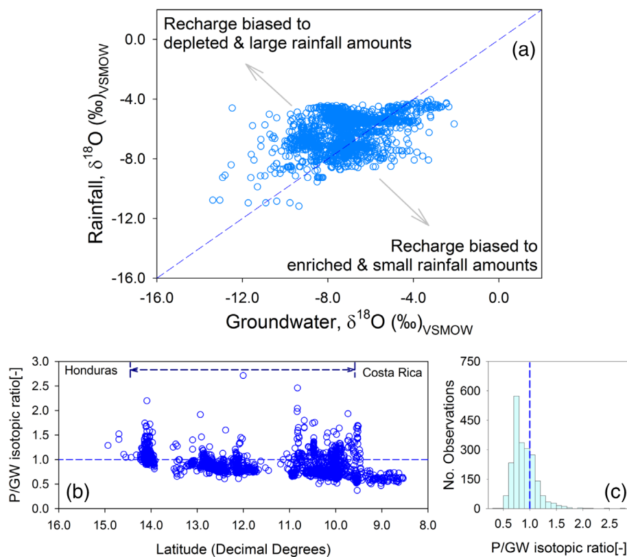
FIGURE 8 Rainfall and groundwater recharge bias across the Central American Isthmus. (a) Rainfall and groundwater recharge bias 1:1 diagram following Jasechko and Taylor (2015). (b) Latitudinal variation of P/GW isotopic ratios [-] from Costa Rica to Honduras. (c) Histogram of P/GW isotopic ratios [-]. In (b) and (c), the blue dashed-line represents a P/GW = 1
