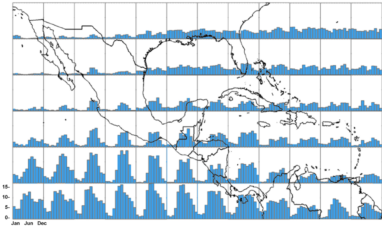
FIGURE 2 Spatial and temporal distribution of rainfall across the Central American Isthmus. Climatology distribution of monthly mean precipitation (in mm/day) for contiguous 5^{\circ} \times 5^{\circ} area boxes for the 1998–2017 period, estimated using the rainfall product 3B43-7 (Huffman et al., 2015)
