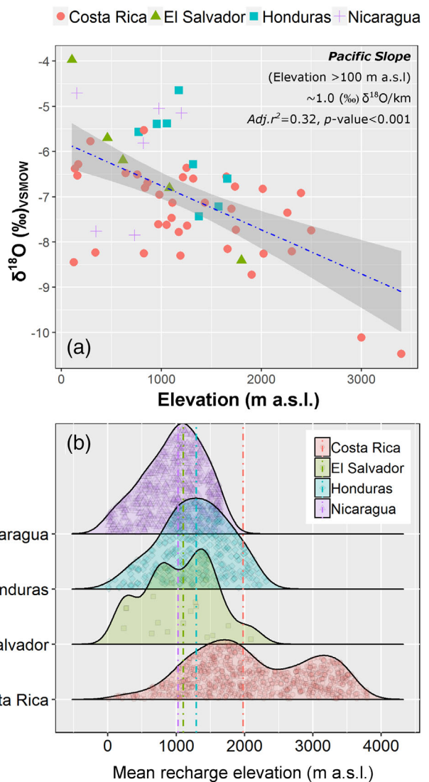
FIGURE 7 Isotopic lapse rates and potential mean recharge elevations (MRE). (a) Regionalized isotopic lapse rate within the Central American Isthmus using monitoring stations above 100 m a.s.l. Blue dashed-line represents the best linear fit resulting in \sim 1\text{‰} \delta^{18}\text{O} per kilometre of elevation gradient with 95% confidence intervals (dark grey area). (b) Density distribution of MRE (m a.s.l.) by country. Dashed coloured-lines denote the median value of each country
