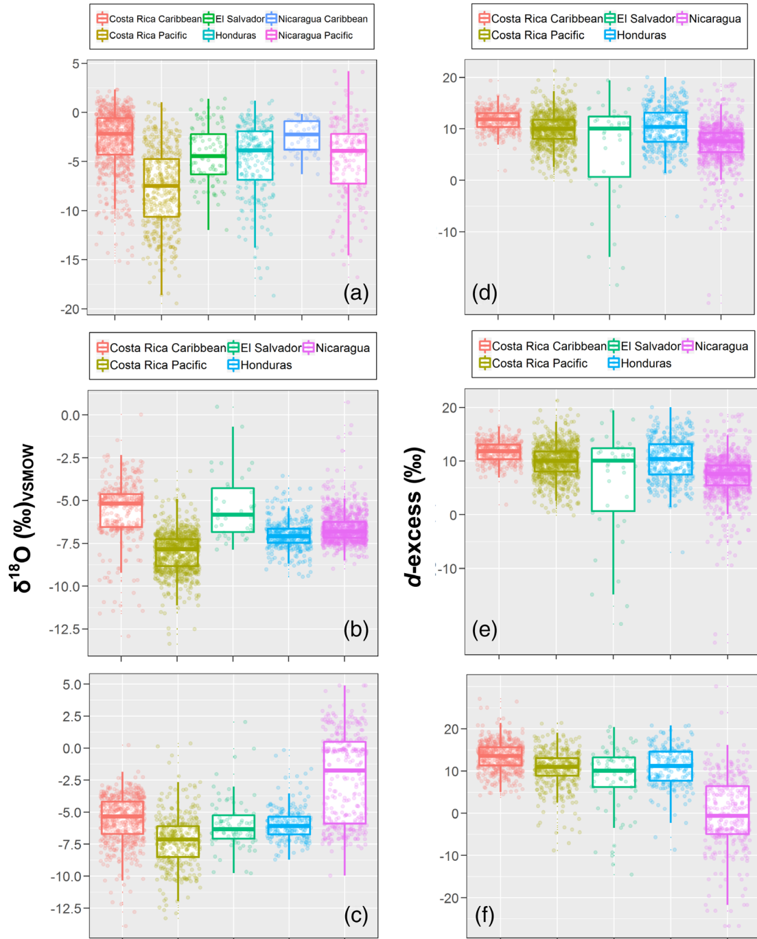
FIGURE 6 Scattered and box plots showing variations across the Central American Isthmus (ordered by country and governing rainfall domain) of (a–c) \delta^{18}\text{O} in rainfall, groundwater, and surface water; and (d–f) d -excess in rainfall, groundwater, and surface water, respectively. Box plots include 25th, 75th, median, and outliers for each group
