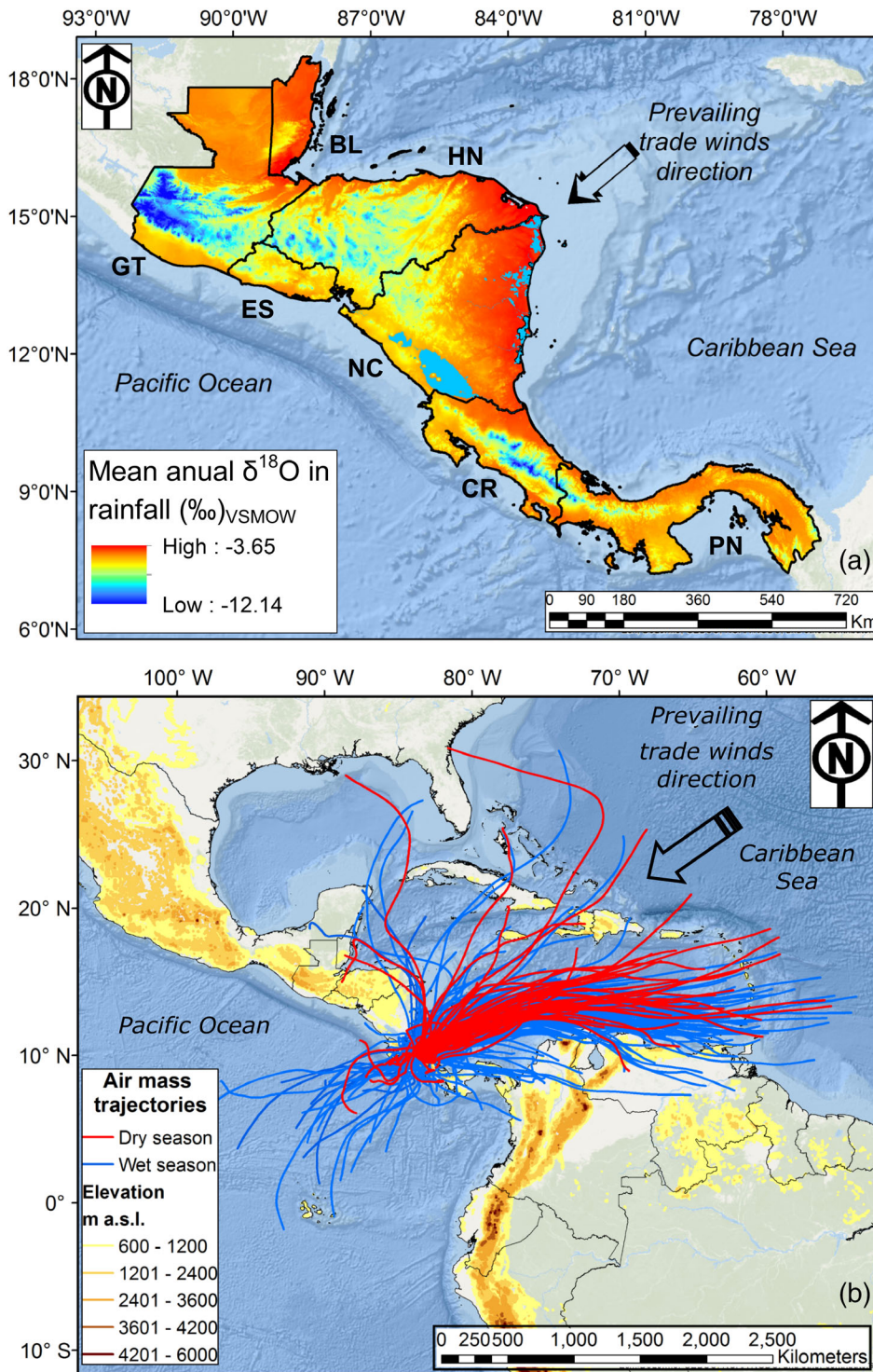
FIGURE 4 Study area characteristics. (a) Regionalized rainfall isoscape within the Central American Isthmus. Mean annual \delta^{18}\text{O} (‰) is colour coded. (b) Representative ( N = 476 ) dry (red) and wet (blue) seasons 48-hr air mass back trajectories over Costa Rica (2013–2017) using the HYSPLIT Lagrangian model (Stein et al., 2015). Trade winds cross Central America with a NE \rightarrow SW prevailing direction, resulting in notable orographic distillation and complex isotopic spatial variations. BL, Belize; CR, Costa Rica; ES, El Salvador; GT, Guatemala; HN, Honduras; NC, Nicaragua; PN, Panama
